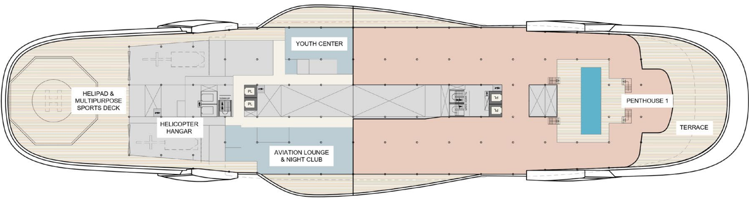
DECK 14
