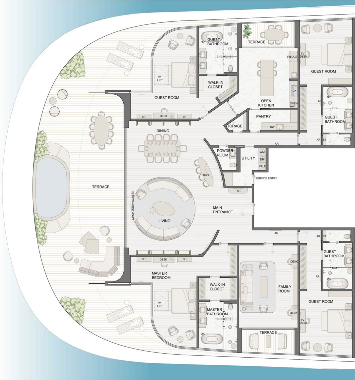
ULYSSIA PENTHOUSE 2 Floor Plan
